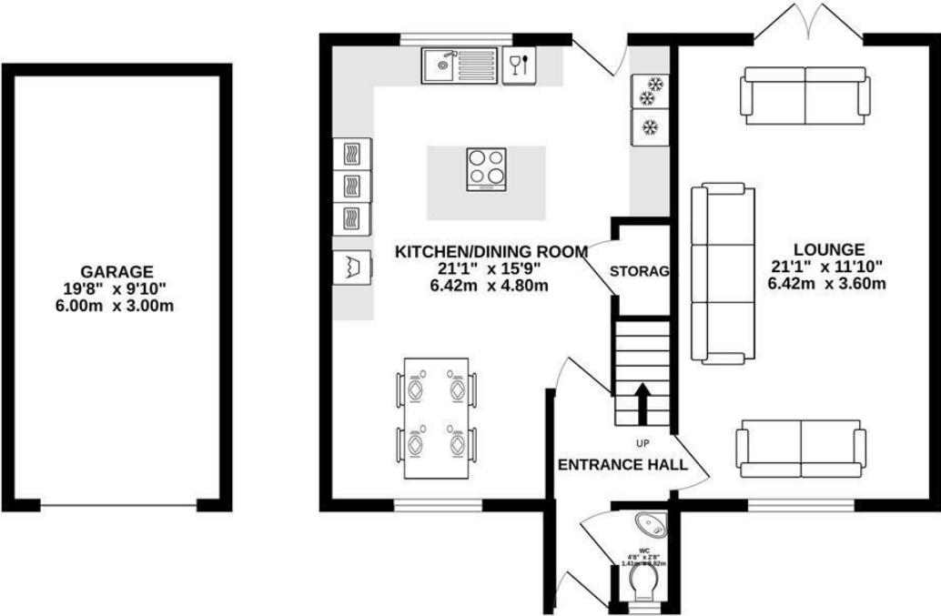
GROUND FLOOR 800 sq.ft. (74.3 sq.m.) approx.
